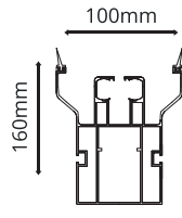
Rafter Thickness : 2mm
