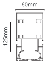
Rafter Profile Thickness : 2mm
