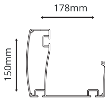
Gutter Profile Thickness : 3mm
