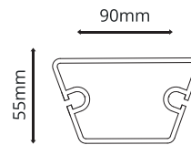
Puller Profile Thickness : 2mm
