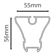
Fabric Support Profile Thickness : 1.5mm
