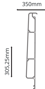
Panel Thickness : 2mm
