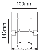
Rafter Profile Thickness : 3mm
