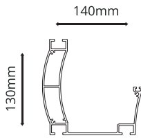
Gutter Profile Thickness : 2mm
