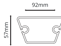
Puller Profile Thickness : 3mm
