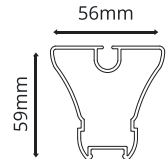
Fabric Support Profile Thickness : 2mm
