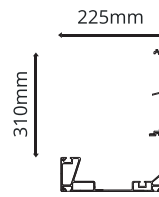
Gutter Profile Thickness : 3mm
